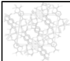
Fig. 2. The polymeric structure of (I) in the unit cell viewed down b . Non-associative H atoms are omitted and hydrogen bonds are shown as dashed lines.
